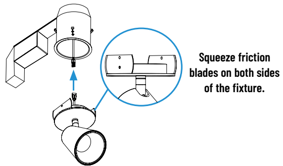
Connect luminaire and install
